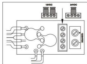
Wiring Instructions
